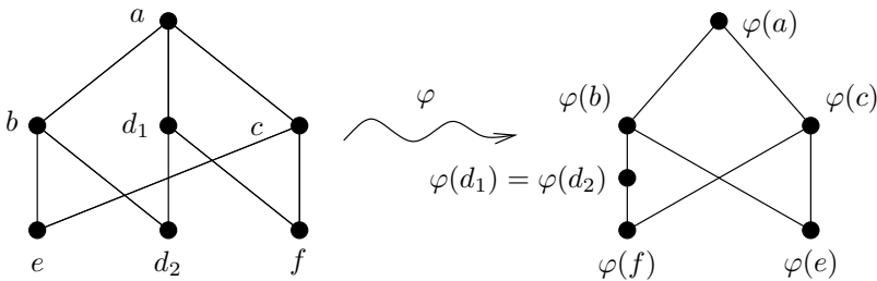
Fig. 11.3. A poset map with small fibers.
