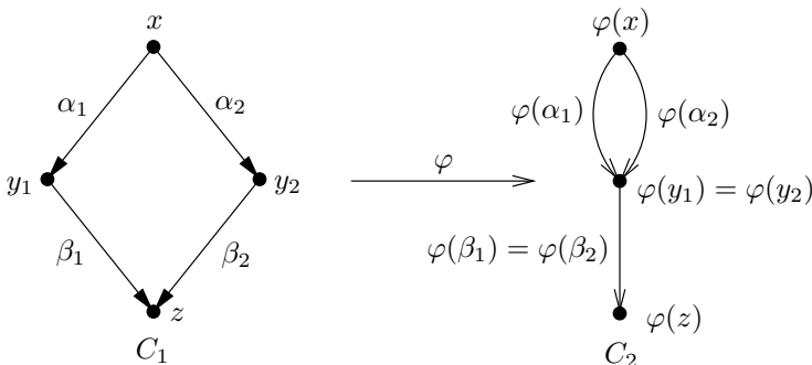
Fig. 10.3. A functor between acyclic categories.
