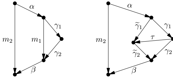
Fig. 10.13. The definition of functor \mathbf{Int}(\alpha, \beta) .
