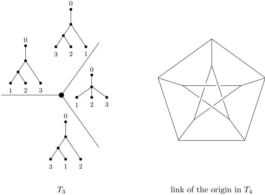
Fig. 9.9. Complexes of phylogenetic trees.
