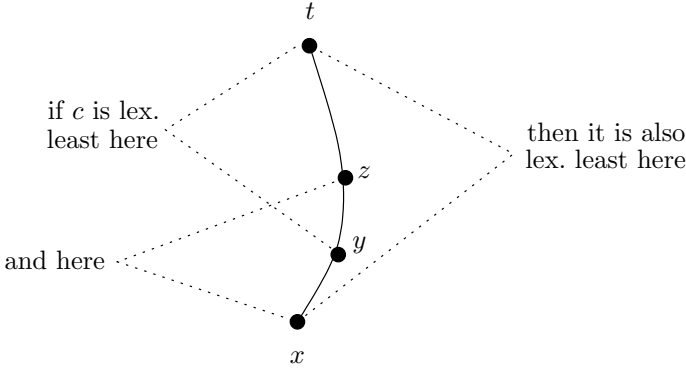
Fig. 12.2. The condition for the lexicographic shelling.
