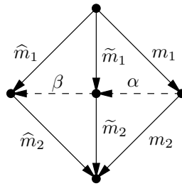
Fig. 10.9. The composition rule in the interval.
