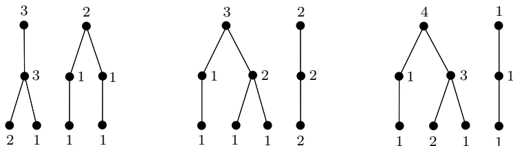
Fig. 11.11. Examples of labeled forests indexing 2-simplices of the generalized simplicial complex \Delta(\bar{I}_n)/\mathcal{S}_n .
