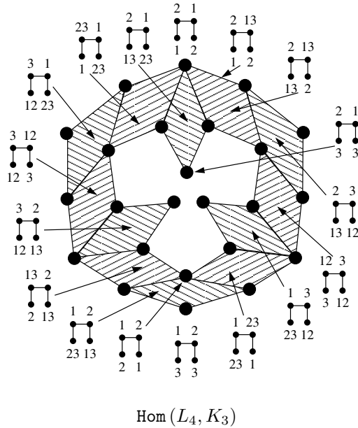
Fig. 18.2. Coloring complexes of strings II.
