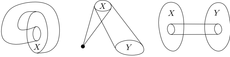
Fig. 15.3. Examples of homotopy colimits.
