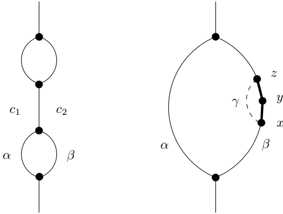
Fig. 12.3. Two maximal chains.
