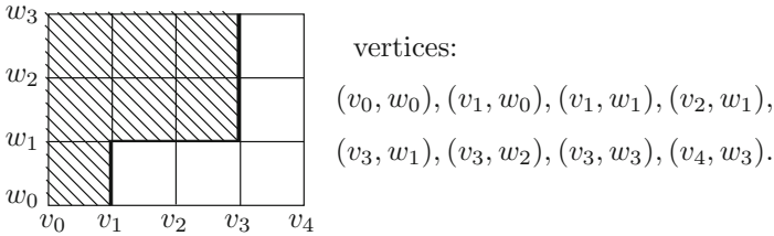
Fig. 64 Triangulation of a product of simplices
