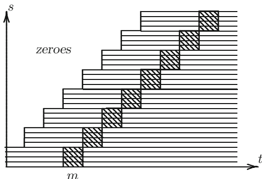
Fig. 122 The structure of the E_\infty -term
