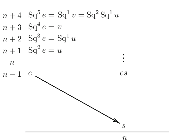
Fig. 110 The spectral sequence of the fibration S^n|_{n+1} \xrightarrow{K(\mathbb{Z}, n-1)} S^n
