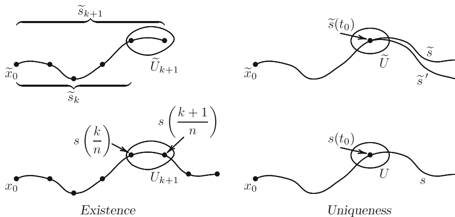
Fig. 26 Proof of the lifting path lemma
