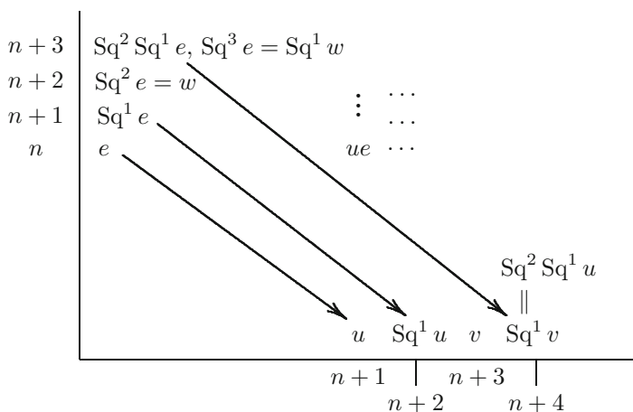
Fig. 111 The spectral sequence of the fibration S^n|_{n+2} \xrightarrow{K(\mathbb{Z}_2, n)} S^n|_{n+1}
