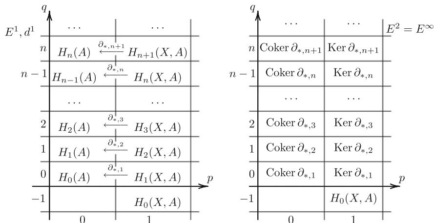
Fig. 79 The spectral sequence of a two-term filtration
