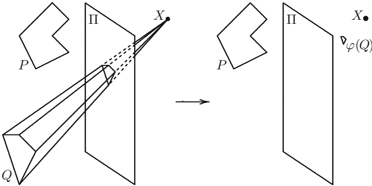
Fig. 51 Separating inverse images of poles
