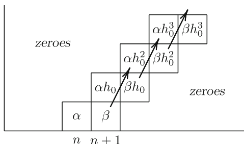
Fig. 130 The Adams spectral sequence for X = K(\mathbb{Z}_4, n)
