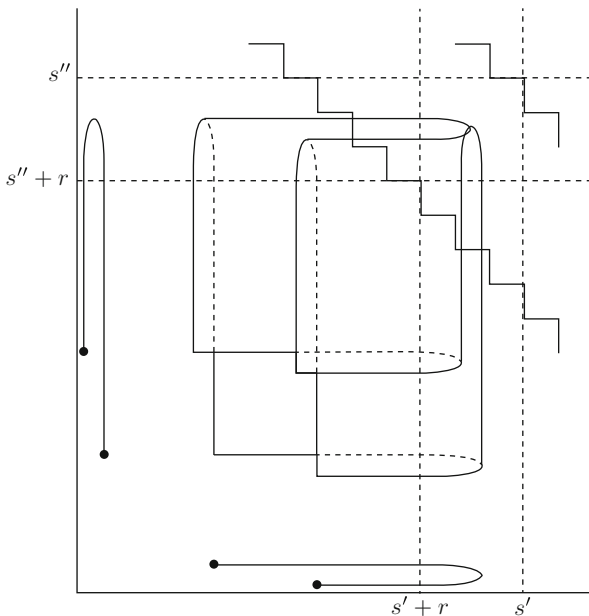
Fig. 125 Product of relative spheroids
