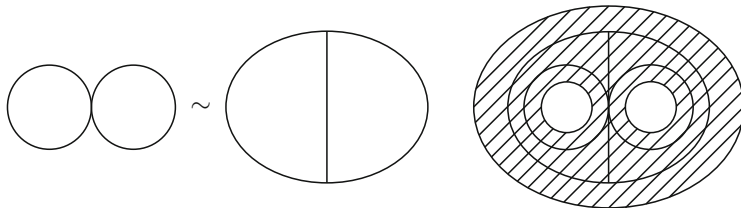
Fig. 11 Homotopy equivalence with no deformation retraction
