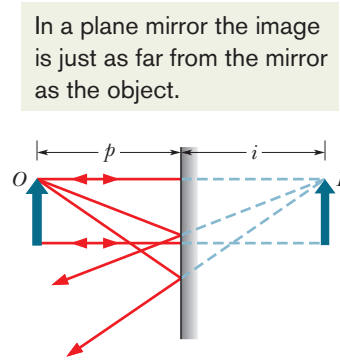
Fig. 34-5 An extended object O and its virtual image I in a plane mirror.
