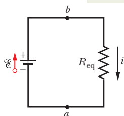
Fig. 27-5 (a) Three resistors are connected in series between points a and b . (b) An equivalent circuit, with the three resistors replaced with their equivalent resistance R_{\text{eq}} .
