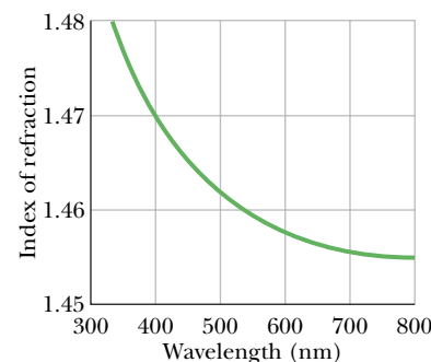
Fig. 33-18 The index of refraction as a function of wavelength for fused quartz. The graph indicates that a beam of short-wavelength light, for which the index of refraction is higher, is bent more upon entering or leaving quartz than a beam of long-wavelength light.
