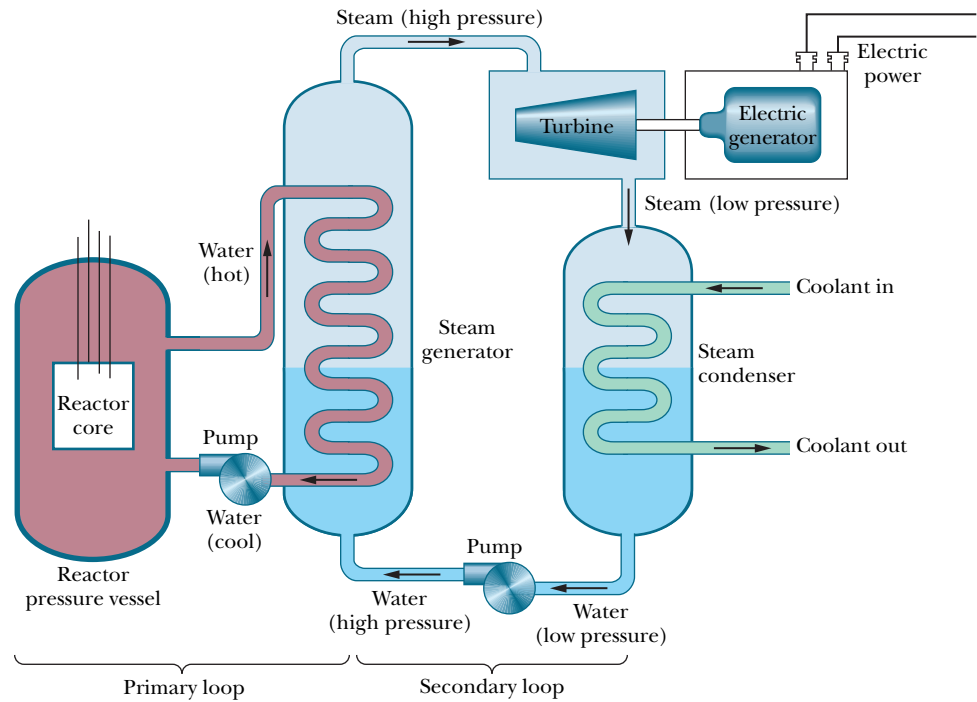
Fig. 43-6 A simplified layout of a nuclear power plant, based on a pressurized-water reactor. Many features are omitted—among them the arrangement for cooling the reactor core in case of an emergency.
