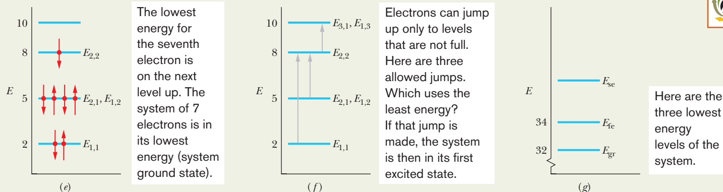
Fig. 40-12 (Continued from page 1123) (e) The system's ground-state configuration. (f) Three transitions to consider for the first excited state. (g) The system's lowest three total energies.
