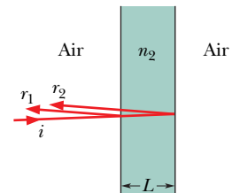
Fig. 35-17 Reflections from a thin film in air.
