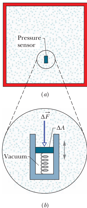
Fig. 14-1 (a) A fluid-filled vessel containing a small pressure sensor, shown in (b). The pressure is measured by the relative position of the movable piston in the sensor.
