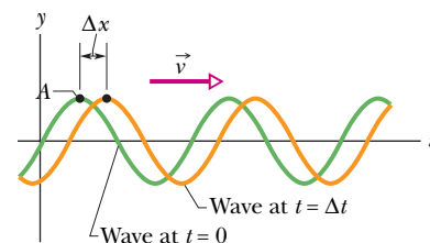
Fig. 16-7 Two snapshots of the wave of Fig. 16-4, at time t = 0 and then at time t = \Delta t . As the wave moves to the right at velocity \vec{v} , the entire curve shifts a distance \Delta x during \Delta t . Point A “rides” with the wave form, but the string elements move only up and down.
