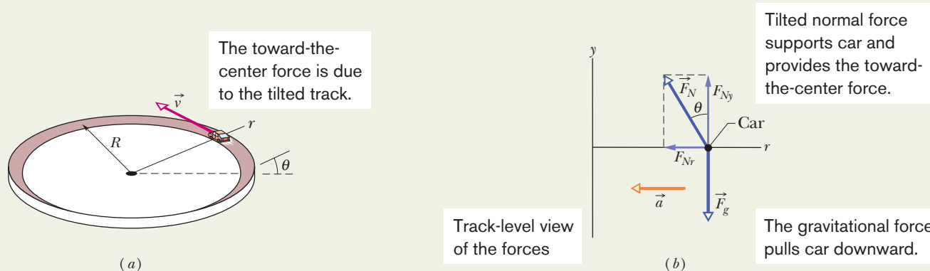
Fig. 6-11 (a) A car moves around a curved banked road at constant speed v . The bank angle is exaggerated for clarity. (b) A free-body diagram for the car, assuming that friction between tires and road is zero and that the car lacks negative lift. The radially inward component F_{Nr} of the normal force (along radial axis r ) provides the necessary centripetal force and radial acceleration.
