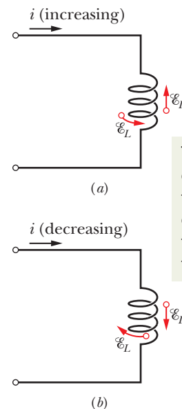
Fig. 30-14 (a) The current i is increasing, and the self-induced emf \mathcal{E}_L appears along the coil in a direction such that it opposes the increase. The arrow representing \mathcal{E}_L can be drawn along a turn of the coil or alongside the coil. Both are shown. (b) The current i is decreasing, and the self-induced emf appears in a direction such that it opposes the decrease.
